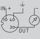
1 (IN) 3 (OUT) 4 (↓)
